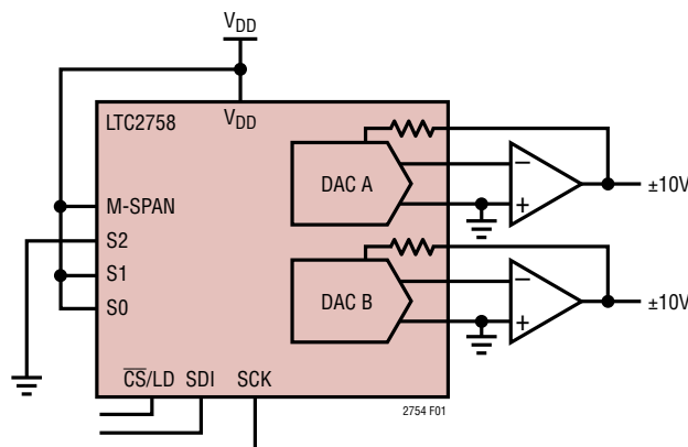
Figure 1. Using M-SPAN to Configure the LTC2758 for Single-Span Operation ( \pm 10\text{V} Range Shown)
