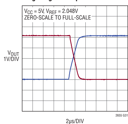
Large-Signal Response
