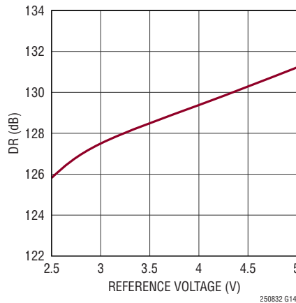
Dynamic Range vs Reference Voltage, f_{IN} = 200\text{Hz} , A_{IN} = -20\text{dBFS}
