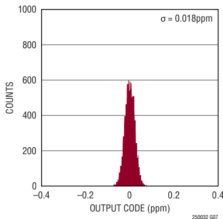
DC Histogram Filtered Output, DF = 16384, SSINC Filter
