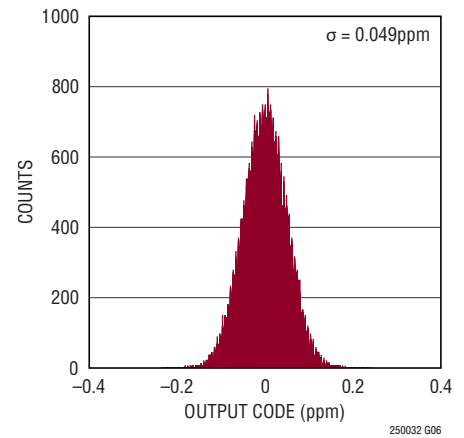
DC Histogram Filtered Output, DF = 1024, SSINC Filter
