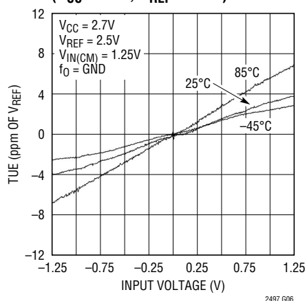
Total Unadjusted Error ( V_{CC} = 2.7V , V_{REF} = 2.5V )
