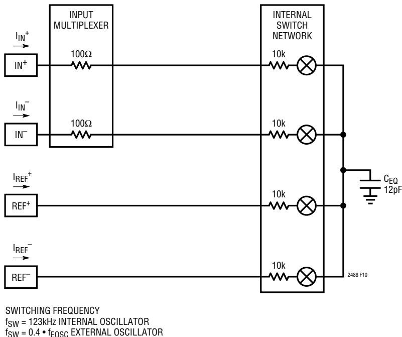
Figure 10. LTC2488 Equivalent Analog Input Circuit
