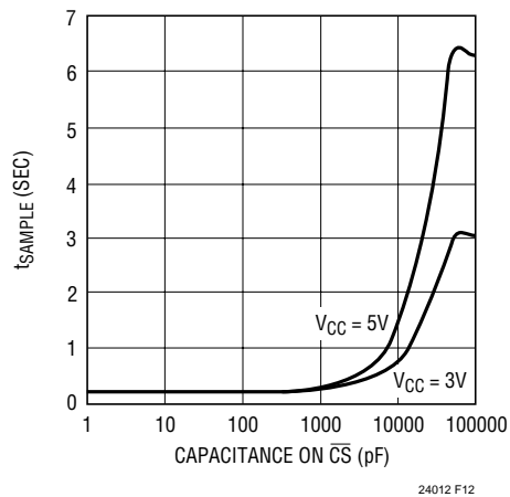
Figure 12. \overline{\text{CS}} Capacitance vs ts SAMPLE
