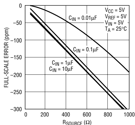
Figure 21. Full-Scale Error vs R_{SOURCE} (Large C)
