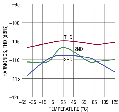
THD, Harmonics at f_{\text{IN}} = 20\text{kHz} vs Temperature
