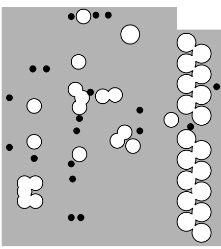
Partial Layer 2 Ground Plane
