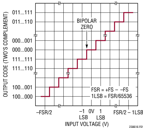
Figure 1. LTC2386-16 Transfer Function
