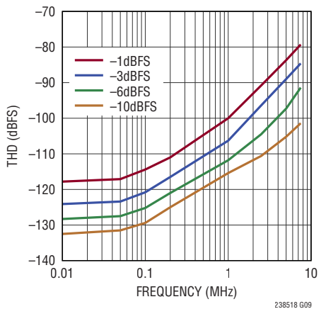
THD vs Input Frequency and Amplitude
