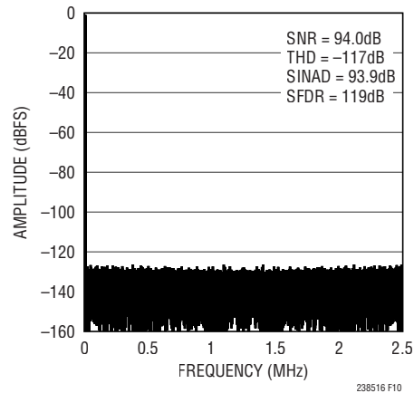
Figure 10. 32k Point FFT of the LTC2385-16, f_{SAMPL} = 5\text{Mps} , f_{IN} = 2\text{kHz}
