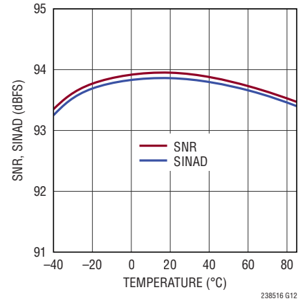
SNR, SINAD vs Temperature, f_{\text{IN}} = 2\text{kHz} , -1\text{dBFS}
