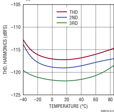
THD, Harmonics vs Temperature, f_{\text{IN}} = 2\text{kHz} , -1\text{dBFS}
