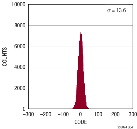
DC Histogram, N = 16, f_{\text{SMPL}} = 2\text{Mps}
