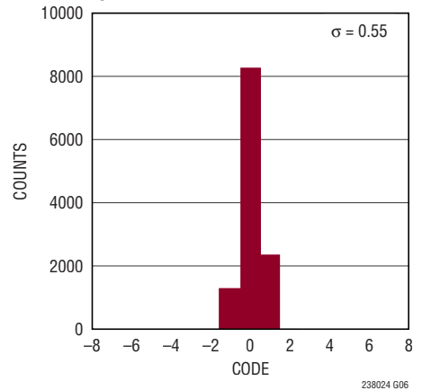
DC Histogram, N = 16384, f_{\text{SMPL}} = 2\text{Mps}
