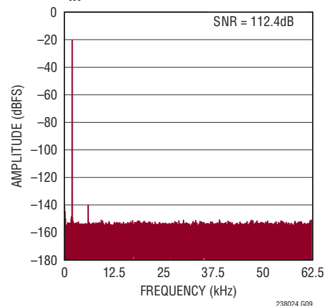
128k Point FFT f_{\text{SMPL}} = 2\text{Mps} , f_{\text{IN}} = 2\text{kHz} , N = 16
