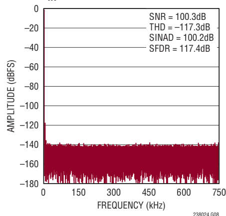
128k Point FFT f_{\text{SMPL}} = 1.5\text{Mps} , f_{\text{IN}} = 2\text{kHz}
