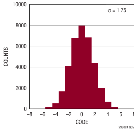
DC Histogram, N = 1024, f_{\text{SMPL}} = 2\text{Mps}
