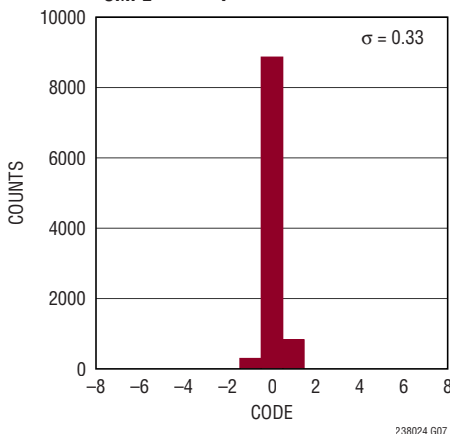
DC Histogram, N = 65536, f_{\text{SMPL}} = 2\text{Mps}
