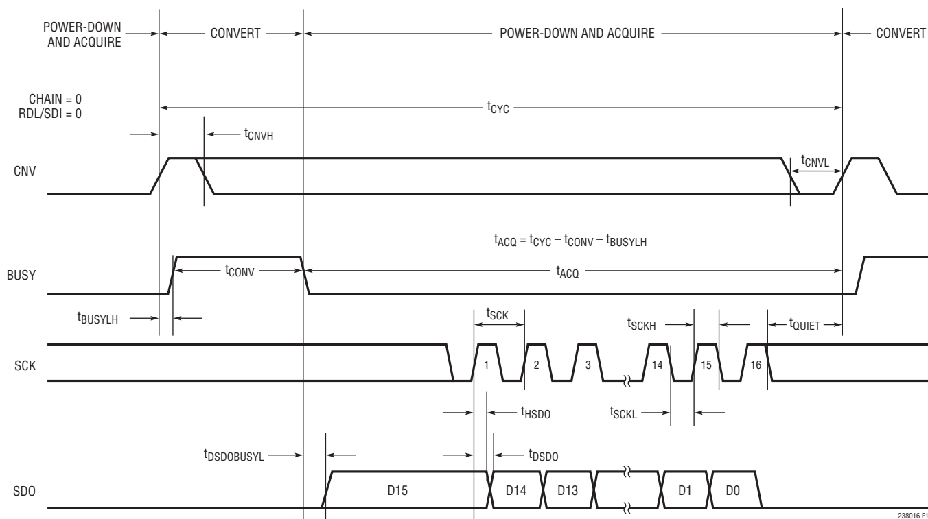
Figure 13. Using a Single LTC2380-16 in Normal Mode
