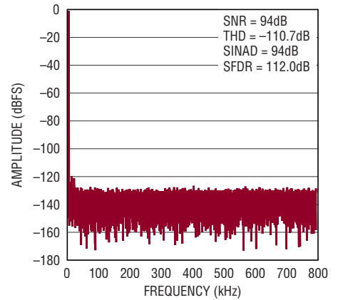
32k Point FFT f_{\text{SAMPL}} = 1.6\text{MSPS} , f_{\text{IN}} = 1\text{kHz} , REFBUF = 5\text{V}
