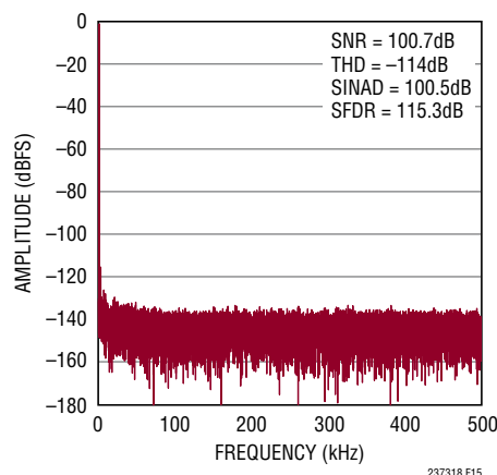
Figure 15. 32k Point FFT f_{SMP} = 1Msps , f_{IN} = 1kHz
