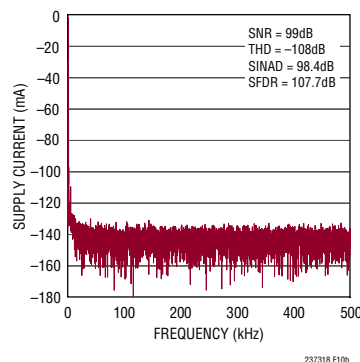
Figure 10b. 32k Point FFT f_{\text{SMPL}} = 1\text{Mps} , f_{\text{IN}} = 1\text{kHz} for Circuit Shown in Figure 10a
