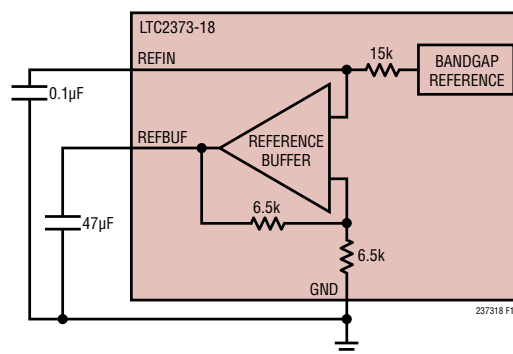
Figure 12a. LTC2373-18 Internal Reference Circuit
