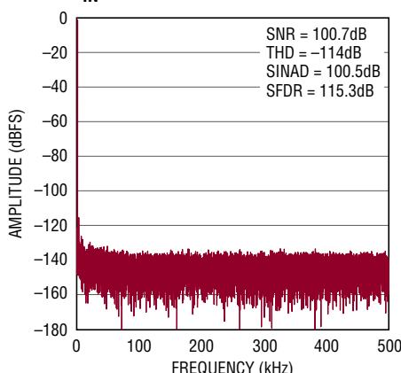
32k Point FFT f_{SAMPL} = 1\text{Mpsps} , f_{IN} = 1\text{kHz}
