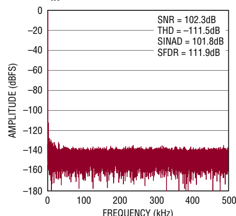
32k Point FFT f_{SAMPL} = 1\text{Mpsps} , f_{IN} = 1\text{kHz} , \text{REFBUF} = 5\text{V}
