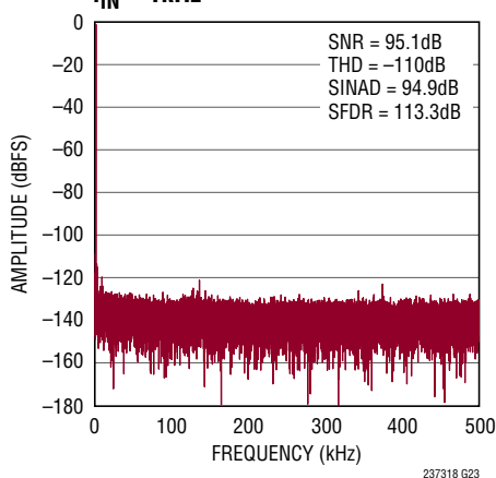
32k Point FFT f_{\text{SAMPL}} = 1\text{Mpsps} , f_{\text{IN}} = 1\text{kHz}
