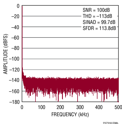
Figure 8b. 32k Point FFT f_{\text{SMP}} = 1\text{Msps} , f_{\text{IN}} = 1\text{kHz} for Circuit Shown in Figure 8a; Driven with Fully Differential Inputs
