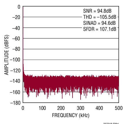
Figure 8d. 32k Point FFT f_{\text{SMP}} = 1\text{Msps} , f_{\text{IN}} = 1\text{kHz} for Circuit Shown in Figure 8a; Driven with Bipolar Inputs
