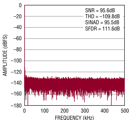
32k Point FFT f_{SAMPL} = 1\text{Mps} , f_{IN} = 1\text{kHz}
