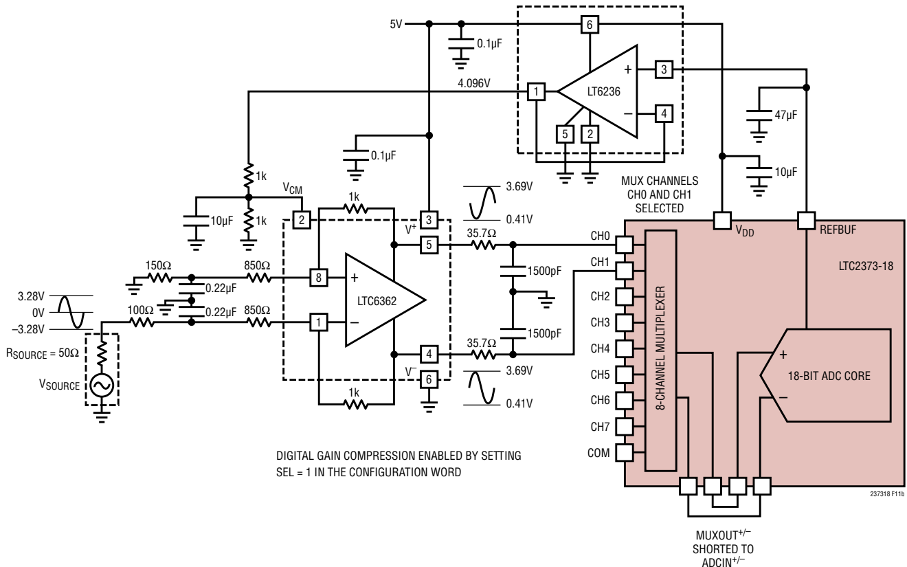
Figure 11b. LTC6362 Configured to Accept a \pm 3.28\text{V} Input Signal While Running from a Single 5V Supply When Digital Gain Compression is Enabled in the LTC2373-18
