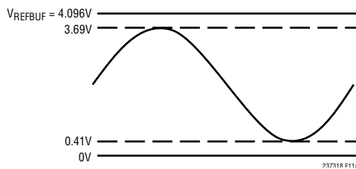
Figure 11a. Input Swing of the LTC2373-18 with Digital Gain Compression Enabled and V_{\text{REFBUF}} = 4.096\text{V}
