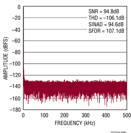
Figure 8c. 32k Point FFT f_{\text{SMPLE}} = 1\text{Msps} , f_{\text{IN}} = 1\text{kHz} for Circuit Shown in Figure 8a; Driven with Unipolar Inputs
