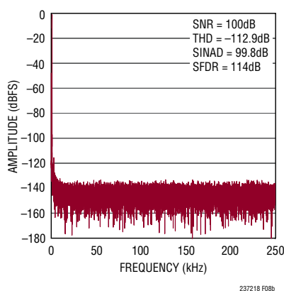
Figure 8b. 32k Point FFT f_{\text{SAMPL}} = 500\text{kps} , f_{\text{IN}} = 1\text{kHz} for Circuit Shown in Figure 8a; Driven with Fully Differential Inputs
