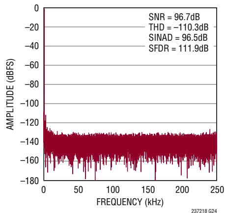
32k Point FFT f_{\text{SAMPL}} = 500\text{kps} , f_{\text{IN}} = 1\text{kHz} , REFBUF = 5\text{V}
