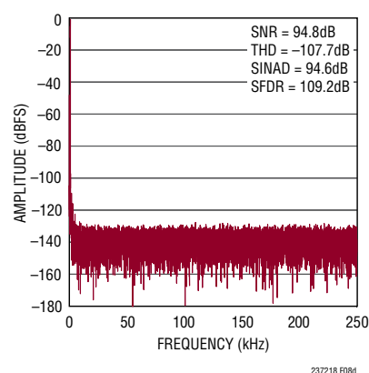
Figure 8d. 32k Point FFT f_{\text{SAMPL}} = 500\text{kps} , f_{\text{IN}} = 1\text{kHz} for Circuit Shown in Figure 8a; Driven with Bipolar Inputs
