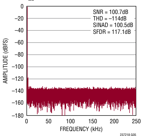
32k Point FFT f_{SAMPL} = 500\text{ksps} , f_{IN} = 1\text{kHz}
