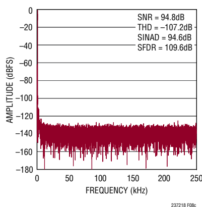
Figure 8c. 32k Point FFT f_{\text{SAMPL}} = 500\text{kps} , f_{\text{IN}} = 1\text{kHz} for Circuit Shown in Figure 8a; Driven with Unipolar Inputs
