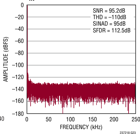
32k Point FFT f_{\text{SAMPL}} = 500\text{kps} , f_{\text{IN}} = 1\text{kHz}
