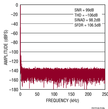
Figure 10b. 32k Point FFT f_{\text{SAMPL}} = 500\text{kpsps} , f_{\text{IN}} = 1\text{kHz} for Circuit Shown in Figure 10a
