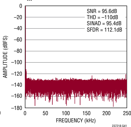
32k Point FFT f_S = 500\text{ksps} , f_{IN} = 1\text{kHz}
