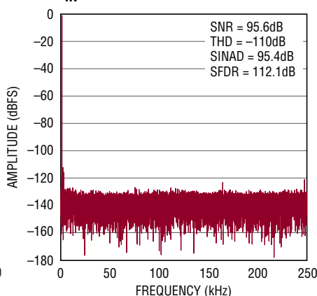
32k Point FFT f_S = 500\text{ksps} , f_{IN} = 1\text{kHz}
