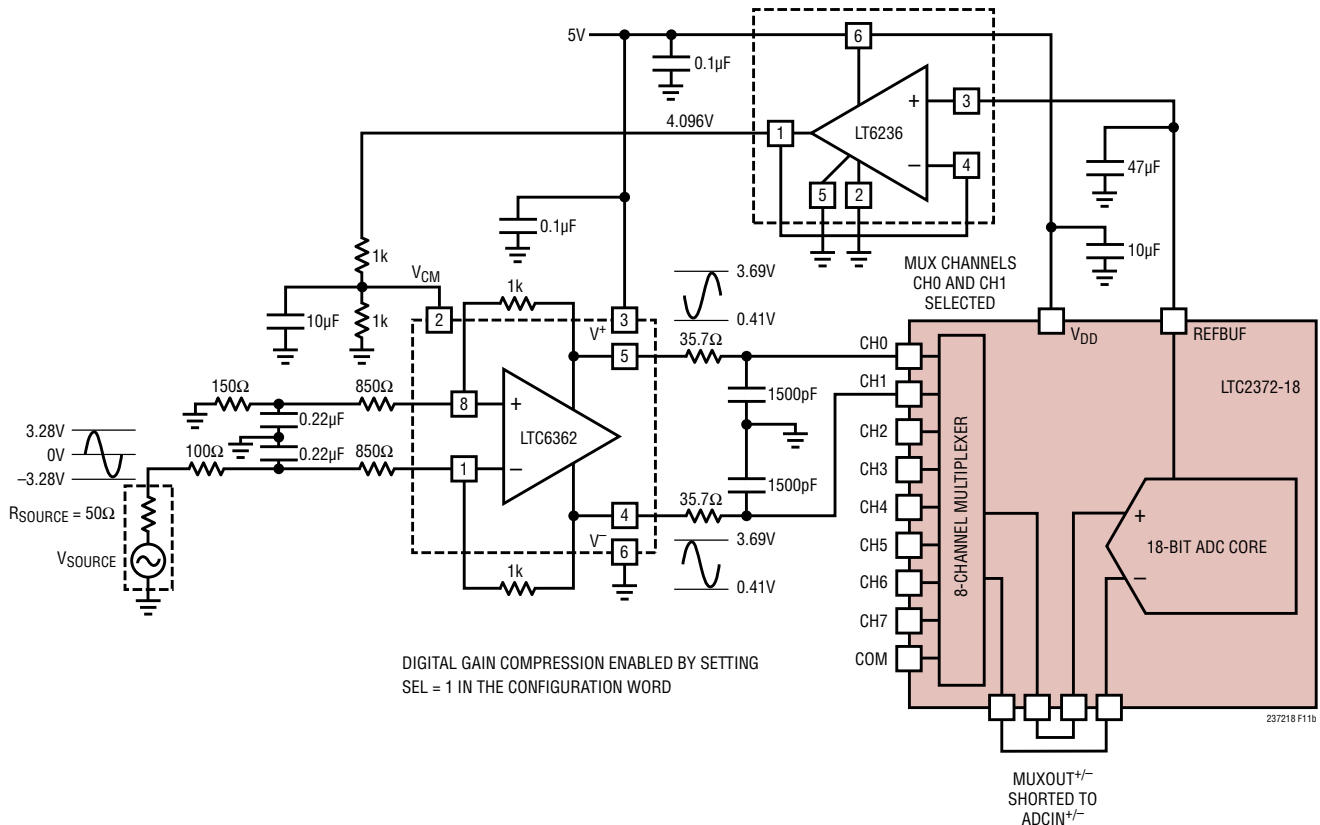
Figure 11b. LTC6362 Configured to Accept a \pm 3.28\text{V} Input Signal While Running from a Single 5V Supply When Digital Gain Compression is Enabled in the LTC2372-18
