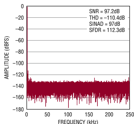
32k Point FFT f_{\text{SAMPL}} = 500\text{ksps} , f_{IN} = 1\text{kHz} , REF_{BUF} = 5\text{V}
