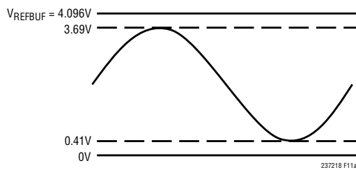
Figure 11a. Input Swing of the LTC2372-18 with Digital Gain Compression Enabled and V_{\text{REFBUF}} = 4.096\text{V}
