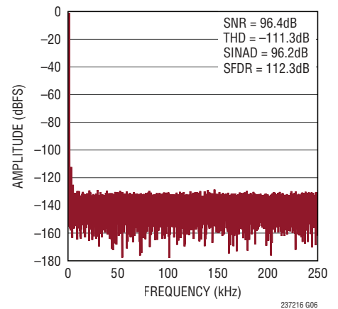
32k Point FFT f_{SAMPL} = 500\text{ksps} , f_{IN} = 1\text{kHz} , REF_{BUF} = 5\text{V}
