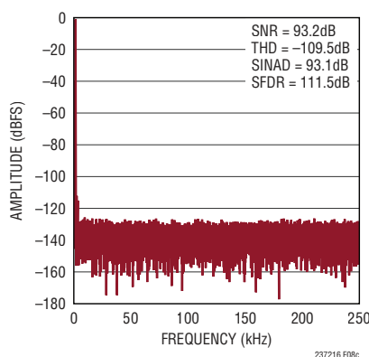
Figure 8c. 32k Point FFT f_{\text{SMPL}} = 500\text{ksps} , f_{\text{IN}} = 1\text{kHz} for Circuit Shown in Figure 8a; Driven with Unipolar Inputs
