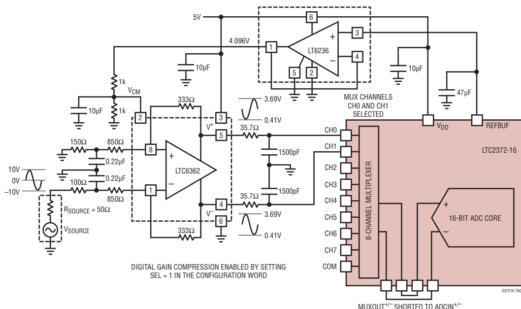
LTC6362 Configured to Accept a \pm 10\text{V} Input Signal Using a Single 5V Supply with Digital Gain Compression Enabled on the LTC2372-16
