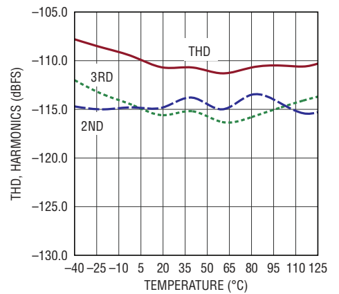
THD, Harmonics vs Temperature, f_{\text{IN}} = 1\text{kHz}
