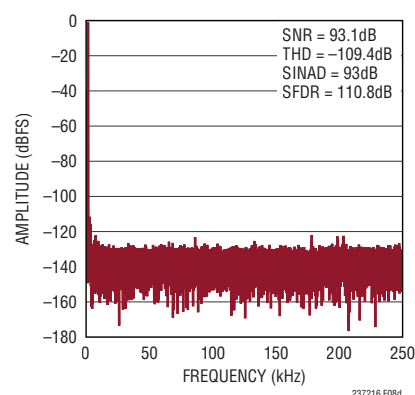
Figure 8d. 32k Point FFT f_{\text{SMPL}} = 500\text{ksps} , f_{\text{IN}} = 1\text{kHz} for Circuit Shown in Figure 8a; Driven with Bipolar Inputs
