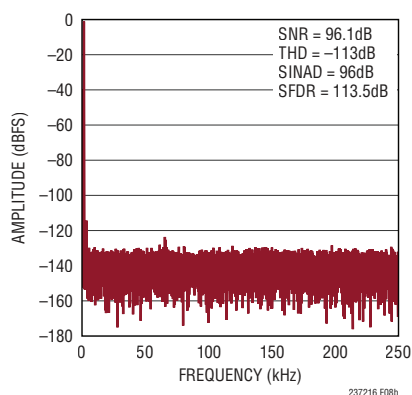
Figure 8b. 32k Point FFT f_{\text{SMPL}} = 500\text{ksps} , f_{\text{IN}} = 1\text{kHz} for Circuit Shown in Figure 8a; Driven with Fully Differential Inputs
