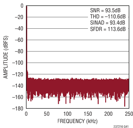
32k Point FFT f_S = 500\text{ksps} , f_{IN} = 1\text{kHz}
