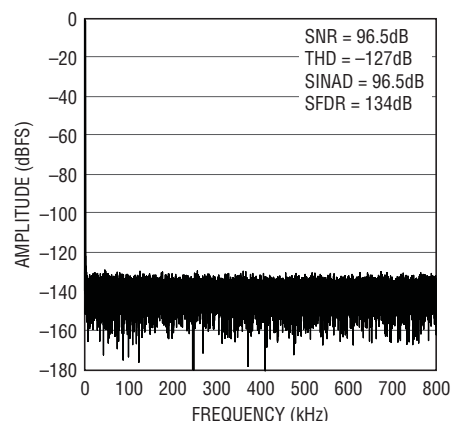
32k Point FFT f_{\text{S}} = 1.6\text{Mps} , f_{\text{IN}} = 2\text{kHz}
