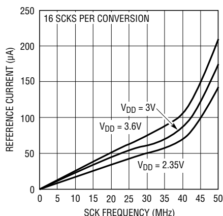
Reference Current vs SCK Frequency (TS8 Package)
