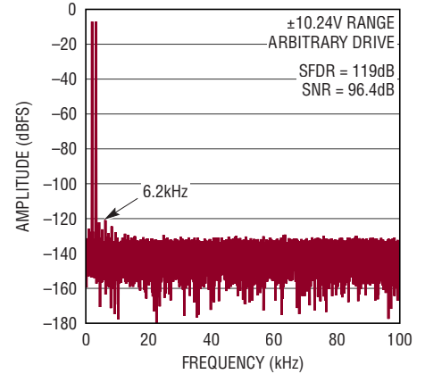
32k Point Arbitrary Two-Tone FFT f_{SAMPL} = 200\text{kHz} , IN^+ = -7\text{dBFS } 2\text{kHz} Sine, IN^- = -7\text{dBFS } 3.1\text{kHz} Sine
