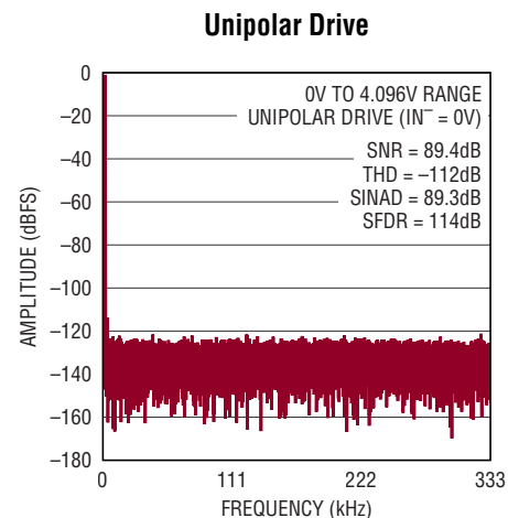
Figure 6e. IN^+ = -1\text{dBFS} 2kHz Unipolar Sine, IN^- = 0\text{V} , 32k Point FFT, f_{\text{SAMPL}} = 666\text{kpsps} . Circuit Shown in Figure 6a with LT6237 Amplifiers, R_{\text{FILT}} = 24.9\Omega , C_{\text{FILT}} = 1\text{nF}
