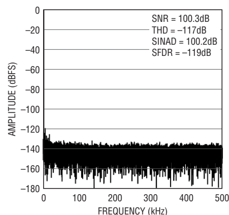
32k Point FFT f_{\text{S}} = 1\text{Msps} , f_{\text{IN}} = 2\text{kHz}
