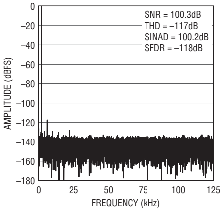
32k Point FFT f_s = 250\text{kpsps} , f_{\text{IN}} = 2\text{kHz}
