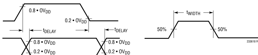
Figure 1. Voltage Levels for Timing Specifications
