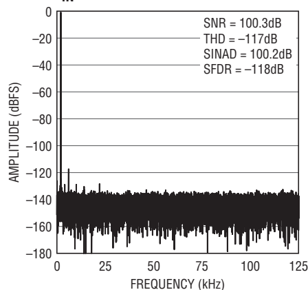
32k Point FFT f_s = 250\text{kpsps} , f_{IN} = 2\text{kHz}
