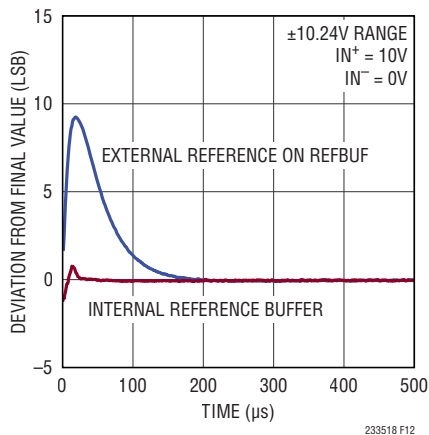
Figure 12. Burst Conversion Response of the LTC2335-18, f_{\text{SAMPL}} = 1\text{Mps}
