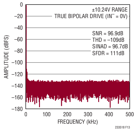
Figure 13. 32k Point FFT f_{\text{SAMPL}} = 1\text{Mps} , f_{\text{IN}} = 2\text{kHz}
