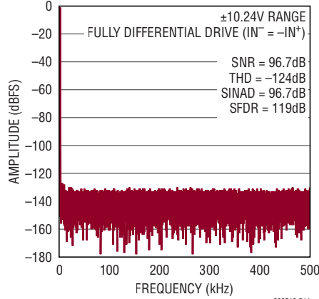
32k Point FFT f_{SAMPL} = 1\text{Mpsps} , f_{IN} = 2\text{kHz}
