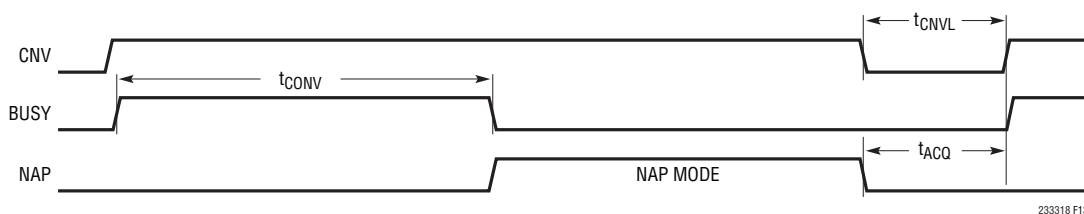
Figure 13. Nap Mode Timing for the LTC2333-18
