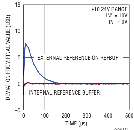
Figure 11. Burst Conversion Response of the LTC2333-18, f_{\text{SMPL}} = 800\text{ksps}
