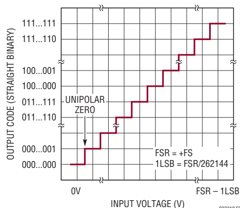
Figure 3. LTC2333-18 Straight Binary Transfer Function
