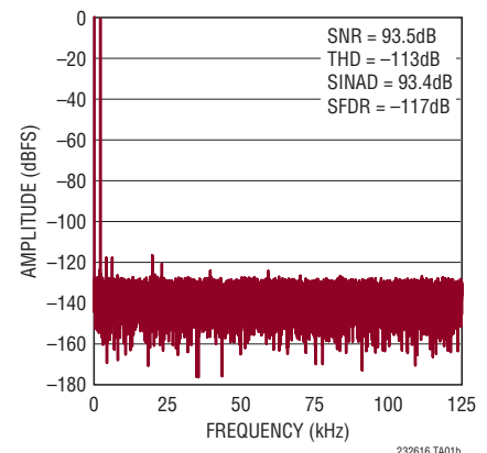
32k Point FFT f_{\text{S}} = 250\text{ksps} , f_{\text{IN}} = 2\text{kHz}
