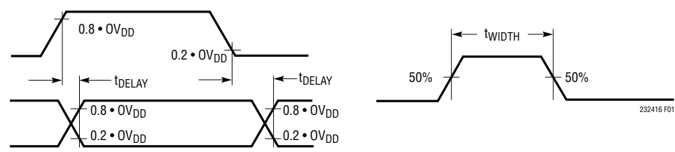
Figure 1. Voltage Levels for Timing Specifications
