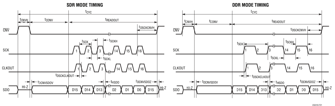
Figure 21. LTC2324-16 Timing Diagram
