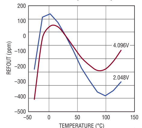
REFOUT1,2 Output vs Temperature
