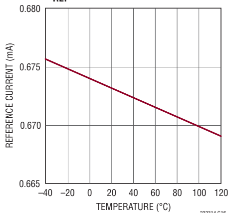
I_{REF} vs Temperature, V_{REF} = 4.096\text{V}
