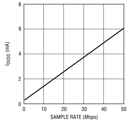
LTC2297: I_{OVD} vs Sample Rate, 5MHz Sine Wave Input, -1dB, O_{VDD} = 1.8\text{V}
