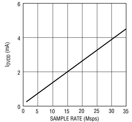
LTC2286: I_{OVD} vs Sample Rate, 5MHz Sine Wave Input, -1dB, O_{VDD} = 1.8\text{V}
