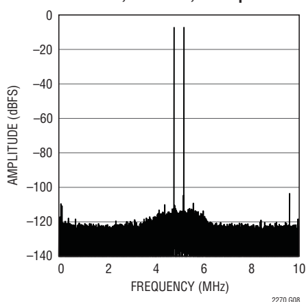
64k Point 2-Tone FFT, f_{IN} = 14.8 , 15.2\text{MHz} , -7dBFS, 20Msps
