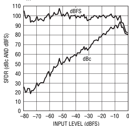
LTC2262-12: SFDR vs Input Level, f_{IN} = 70\text{MHz}, 2\text{V Range}, 150\text{Mps}
