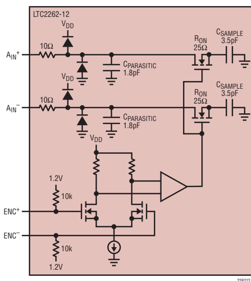
Figure 2. Equivalent Input Circuit
