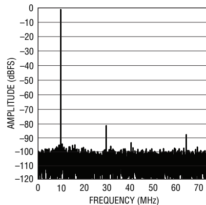
LTC2262-12: 8k Point FFT, f_{IN} = 140\text{MHz} -1dBFS, 150Mps
