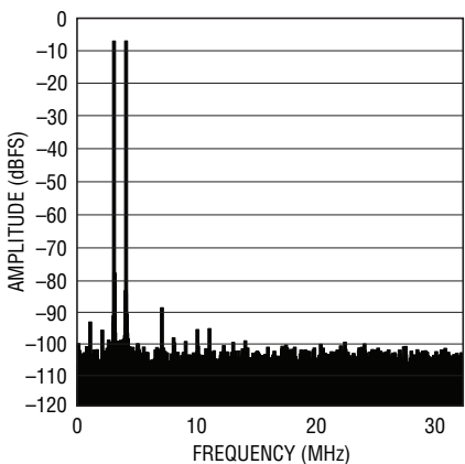
LTC2258-14: 8k Point 2-Tone FFT, f_{IN} = 68\text{MHz} , 69MHz, -1\text{dBFS} , 65Mps
