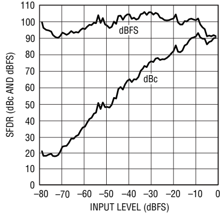
LTC2258-12: SFDR vs Input Level, f_{IN} = 70\text{MHz} , 2V Range, 65Mps
