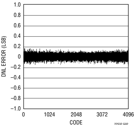
LTC2253: Typical DNL, 2V Range, 125Msps
