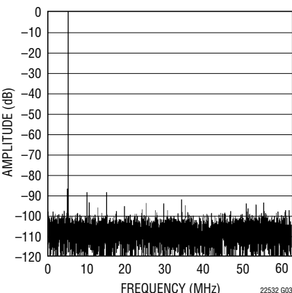
LTC2253: 8192 Point FFT, f_{IN} = 5\text{MHz} , -1dB, 2V Range, 125Msps
