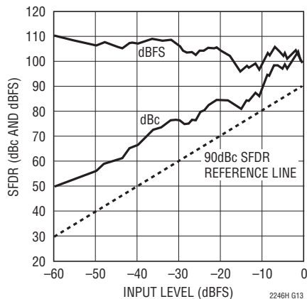
SFDR vs Input Level, f_{IN} = 5\text{MHz} , 2V Range, 25Mps
