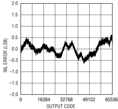
LTC2215 Integral Nonlinearity (INL) vs Output Code, Dither "On"
