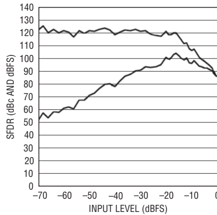
LTC2207: SFDR vs Input Level, f_{IN} = 140\text{MHz} , \text{PGA} = 1 , Dither "On", 105Msps
