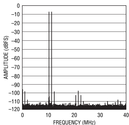
LTC2183: 64k Point 2-Tone FFT, f_{IN} = 69\text{MHz}, 70\text{MHz}, -7\text{dBFS}, 80Mps
