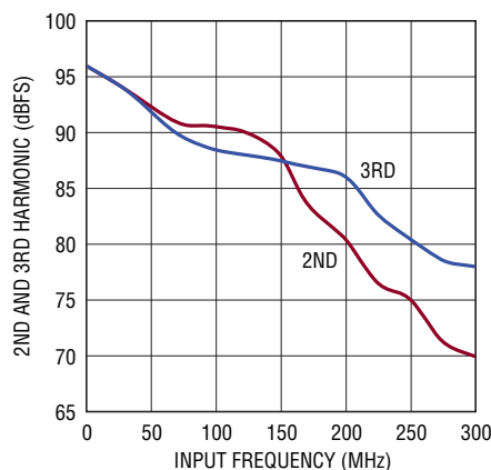
LTC2183: 2nd, 3rd Harmonic vs Input Frequency, -1\text{dBFS}, 80\text{Mps}, 2V Range
