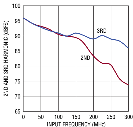
LTC2183: 2nd, 3rd Harmonic vs Input Frequency, -1\text{dBFS}, 80\text{Mps}, 1V Range
