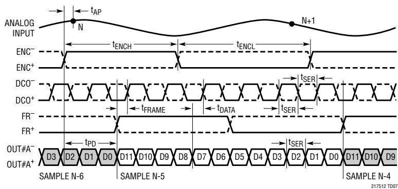
One-Lane Output Mode, 12-Bit Serialization
