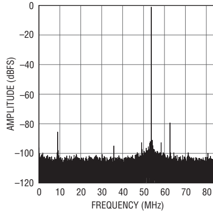
LTC2155-12: 32K Point FFT, f_{IN} = 225\text{MHz} , -1\text{dBFS} , 170Msps
