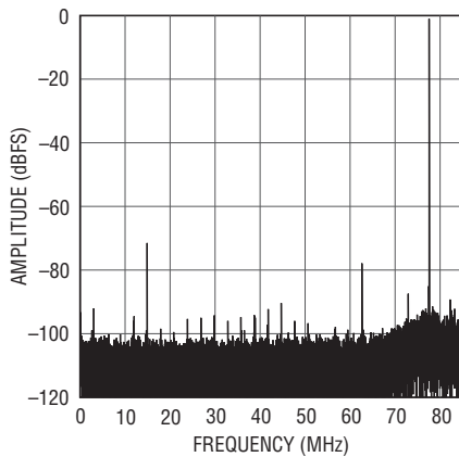
LTC2155-12: 32K Point FFT, f_{IN} = 420\text{MHz} , -1\text{dBFS} , 170Msps
