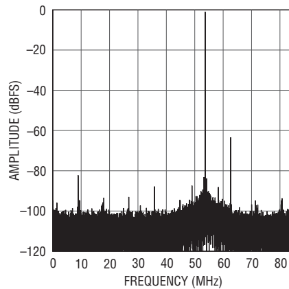
LTC2155-12: 32K Point FFT, f_{IN} = 567\text{MHz} , -1\text{dBFS} , 170Msps
