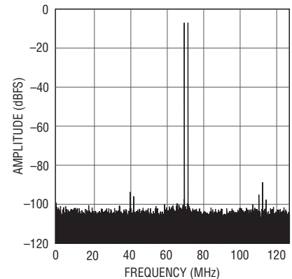
LTC2157-12: 32K Points 2-Tone FFT, f_{\text{IN}} = 71\text{MHz} and 69\text{MHz} , 250Msps
