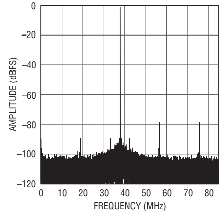
LTC2155-12: 32K Point FFT, f_{IN} = 380\text{MHz} , -1\text{dBFS} , 170Msps
