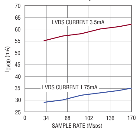
LTC2155-12: I_{OVD} vs Sample Rate, 15MHz Sine Wave Input, -1\text{dBFS}
