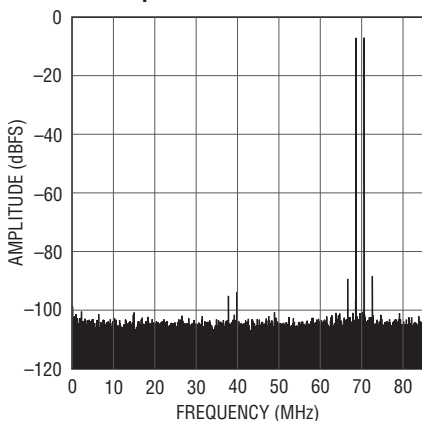
LTC2155-12: 32K Point 2-Tone FFT, f_{IN} = 70.0\text{MHz} and 69.0\text{MHz} , 170Msps
