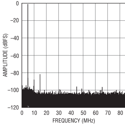
LTC2155-12: 32K Point FFT, f_{IN} = 176\text{MHz} , -1\text{dBFS} , 170Msps
