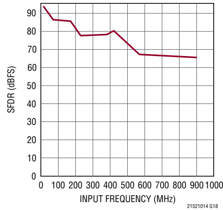
LTC2152-14: SFDR vs Input Frequency, -1dBFS, 1.5V Range, 250Msps
