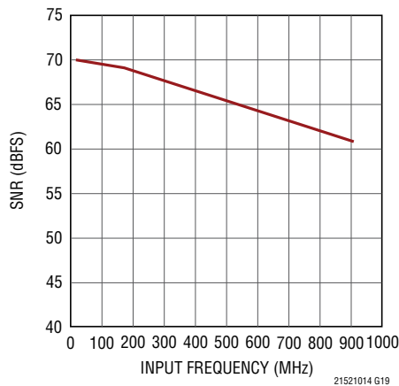
LTC2152-14: SNR vs Input Frequency, -1dBFS, 1.5V Range, 250Msps
